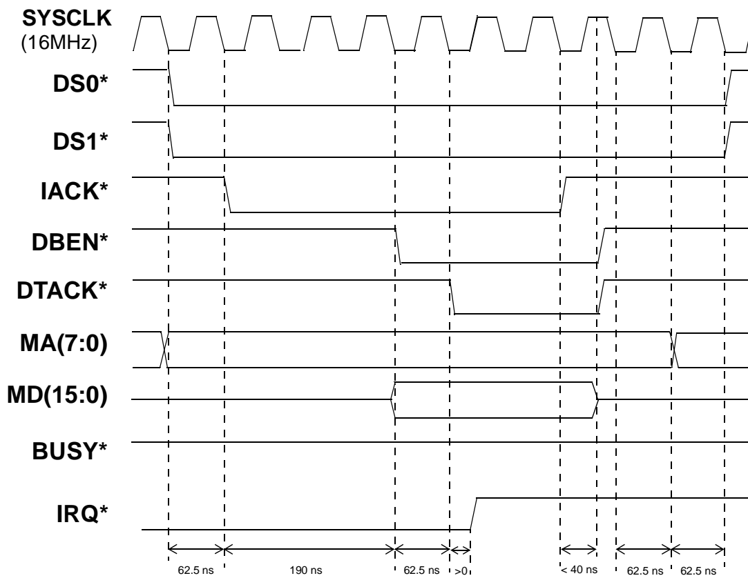
Figure 2-4. Timing for Interrupt Acknowledge Cycle
