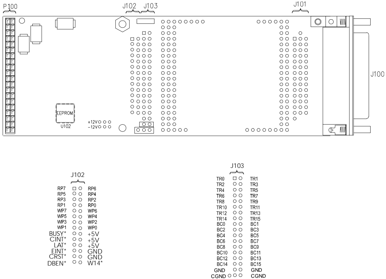
Figure 1-4. J102, J103 Connector Pinouts
