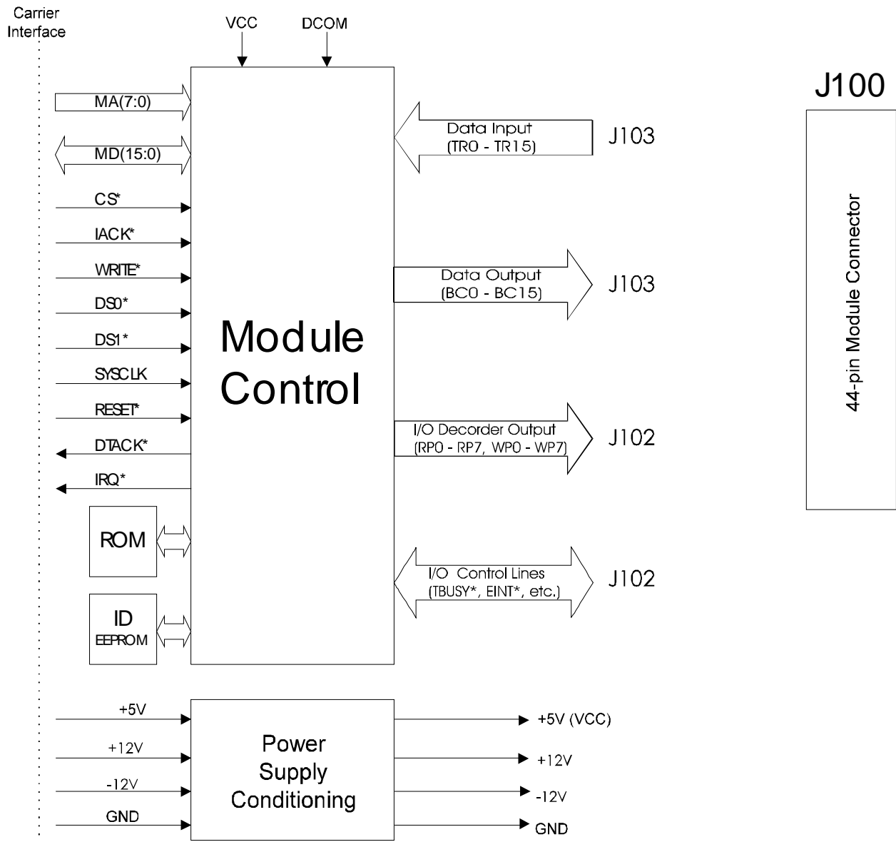
Figure 1-1. Agilent E2259A Block Diagram
