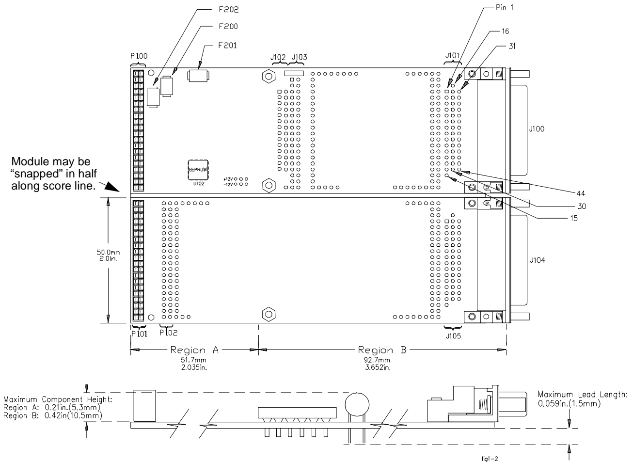
Figure 1-2. Agilent E2259A Connectors Layout
